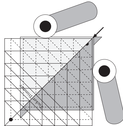
First Trimdown
